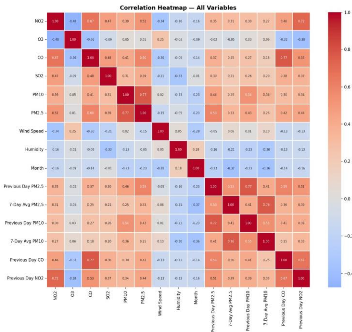
Fig. 4: Correlation heatmap
