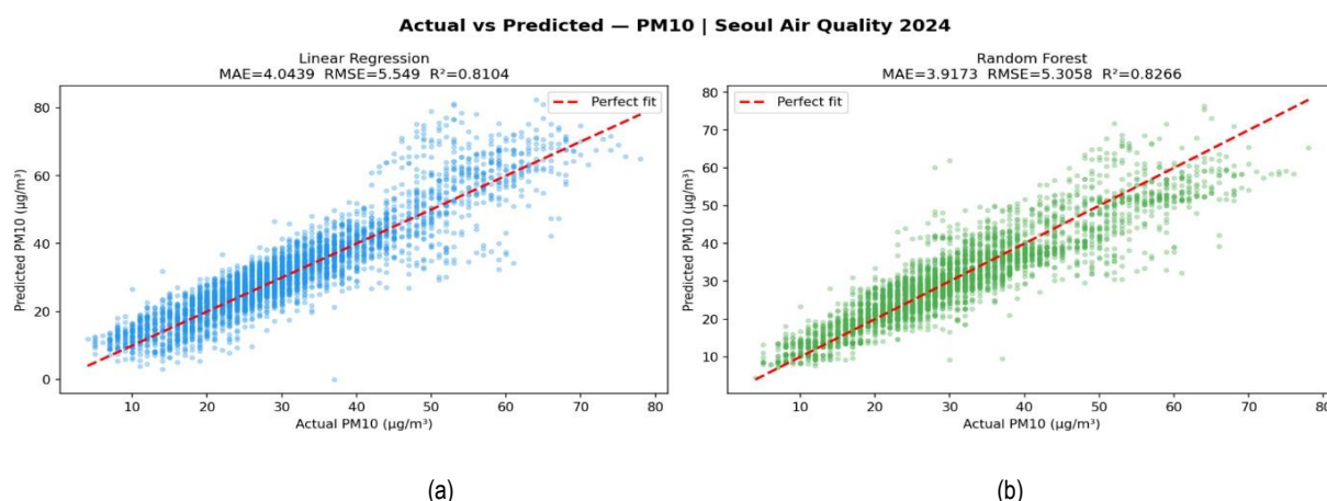
Fig. 2. (a) Linear Regression Actual vs Predicted PM10; (b) Random Forest Actual vs Predicted PM10
