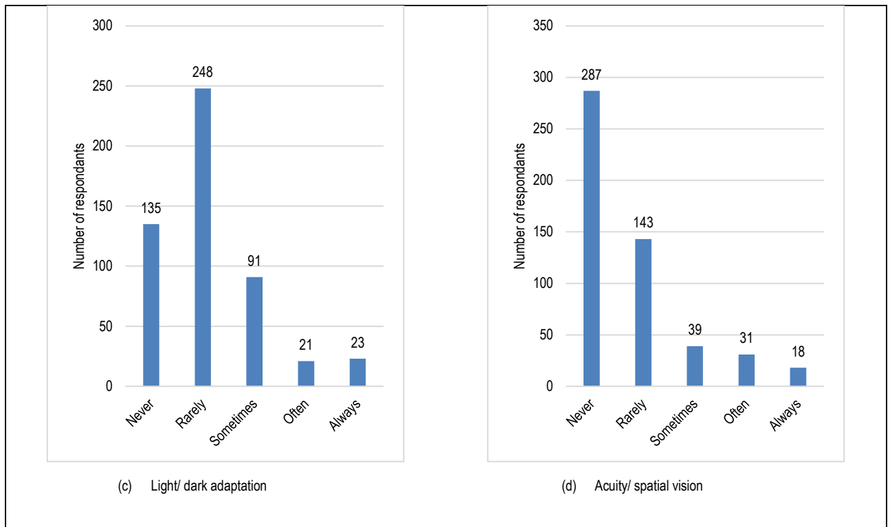
Fig 2: Response of VAQ of selected visual function items, (a) Response on color discrimination; (b) Response on glare disability; (c) Response on light/dark adaptation; and (d) Response on acuity/spatial vision
