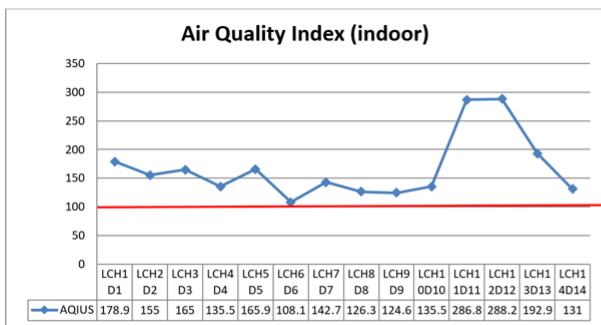
Figure 9: AQI of houses in neighbourhood LC
