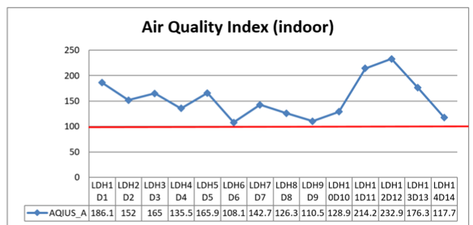
Figure 10: AQI of houses in neighbourhood LD
