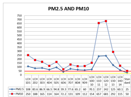
Figure 5: PM exposure of occupants in neighbourhood LC
