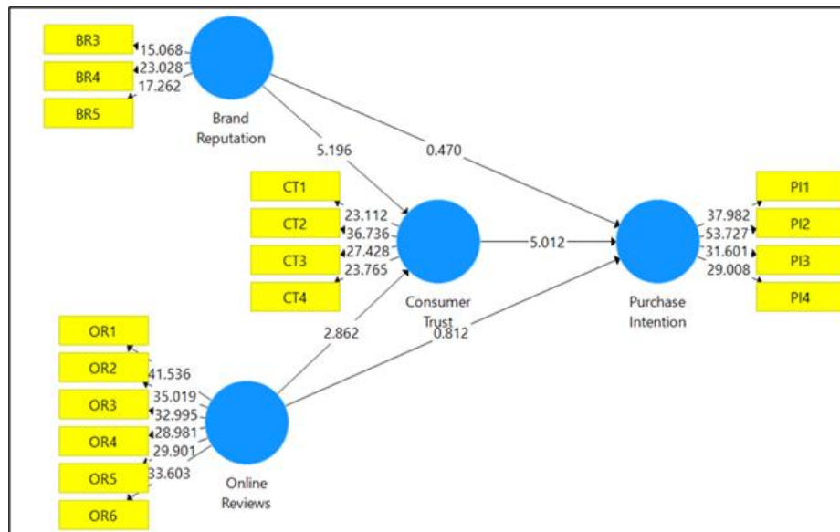
Figure 2: Path Coefficient
